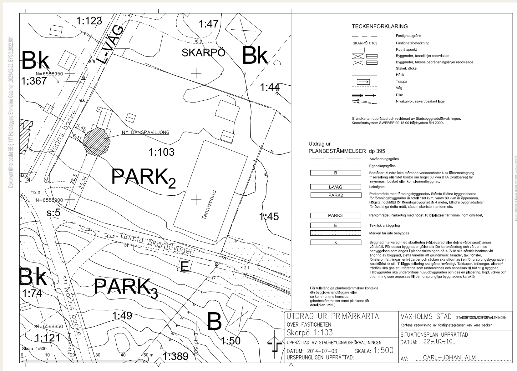
Situationsplan
